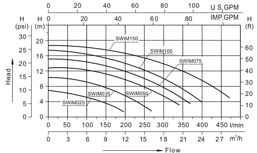
Performance curves
